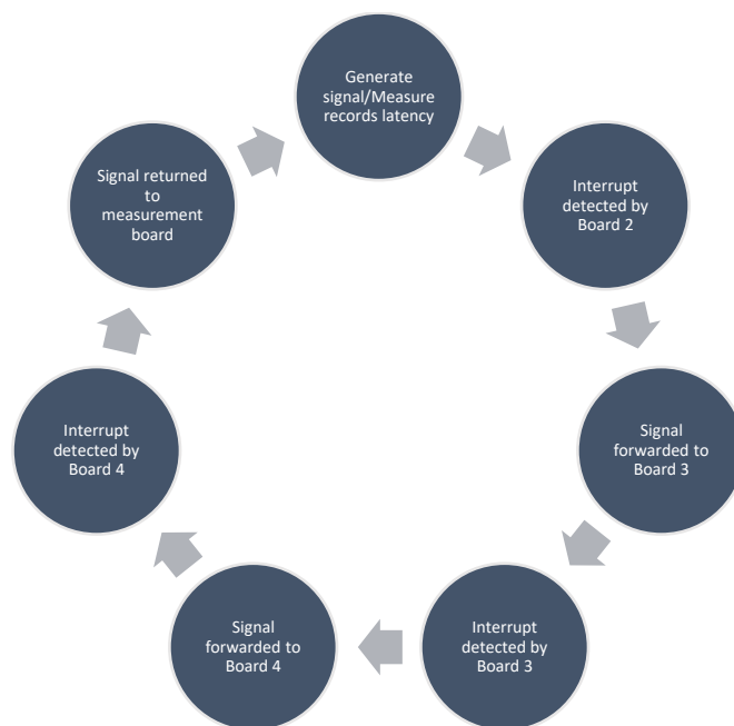
Figure 4.2- Architecture of RTOS-Snake
